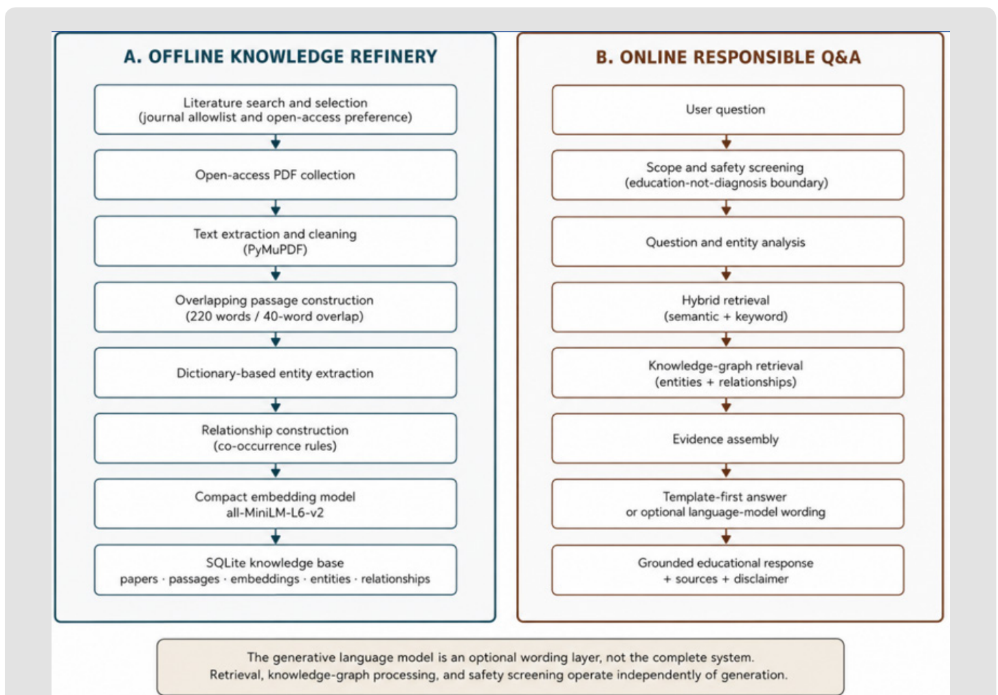
Figure 2: End-to-end architecture of the frugal and responsible DR clinical assistant.
