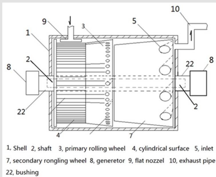
Figure 7: Overall schematic of the proposed steam power-generation device, including the shell, shaft, flat nozzle, primary rolling wheel, secondary rolling wheel, bushings, generator, and exhaust pipe.
