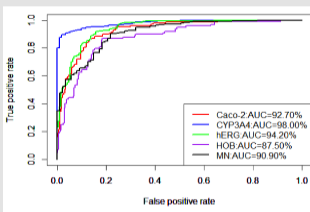
(c) GBM-ROC.
