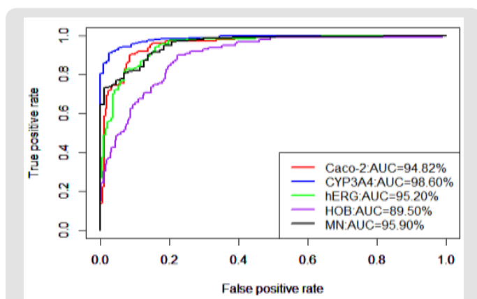
(a) XGBoost-ROC.
