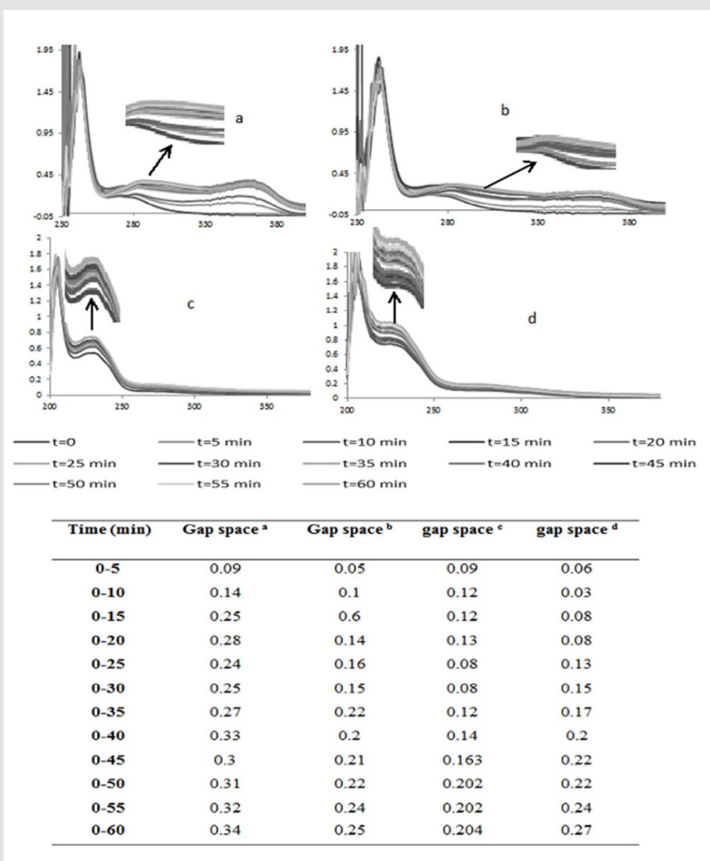
Figure 4: UV-visible spectra and absorption gap spaces of (a) Oleic acid oxidation process by OH•. (b) Oleic acid oxidation process by OH• in the presence of cumin. (c) Oleic acid oxidation process by H 2 O 2 (d) oleic acid oxidation process by H 2 O 2 in the presence of cumin.
