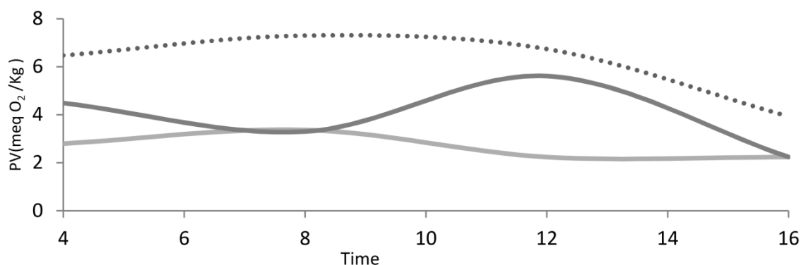
Figure 5: Oleic acid oxidation by superoxide anion radical in the absence of antioxidant (dotted line), oleic acid oxidation in the presence of cumin (contains 6.9 mg polyphenolic compounds) (light gray line) and oleic acid oxidation in the presence of vitamin E (contains 20 mg of natural alpha-tocopherol) (dark gray line).
