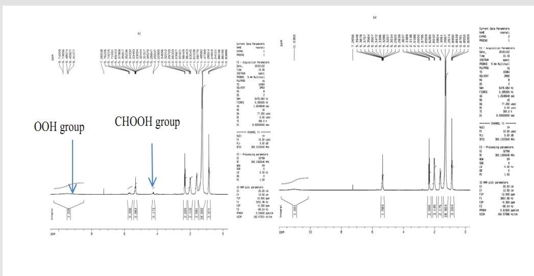
Figure 2: H NMR spectra of oleic acid after photooxygenation in the absence (right) and in the presence (left) of H2TPP as a photosensitizer.
