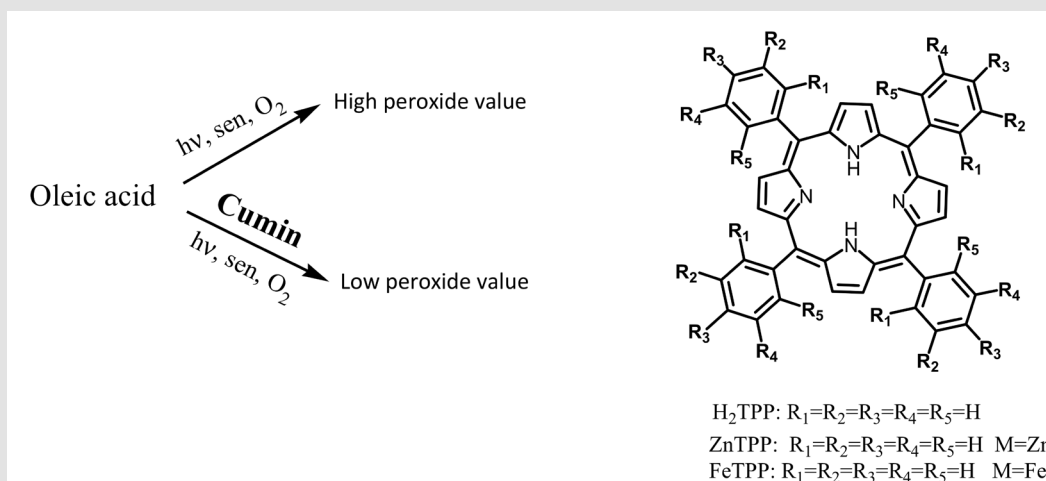
Figure 1: Oleic acid photooxygenation in the presence and absence of cumin antioxidant with photosensitizers (sen) and structure of different applied photosensitizers.
