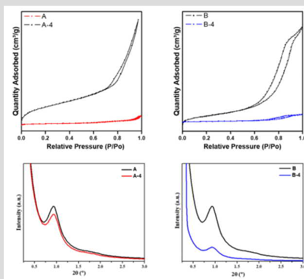
Figure 1: (up) Nitrogen adsorption/desorption isotherms and (down) Small-angle X-ray scattering patterns of the silica and alumina materials A: Silica; B: Alumina; 1: vanillin; 2: eugenol; 3: bis-vanillin; 4: bis-eugenol .
