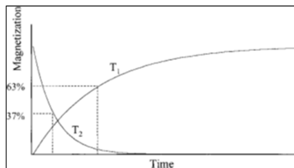
Figure 4: The longitudinal magnetization recovery and transverse magnetization decay occur independently of each other. T_1 is the time to regain 63% of original net magnetization. T_2 is the time of signal decay to 37% of its original signal [2].
