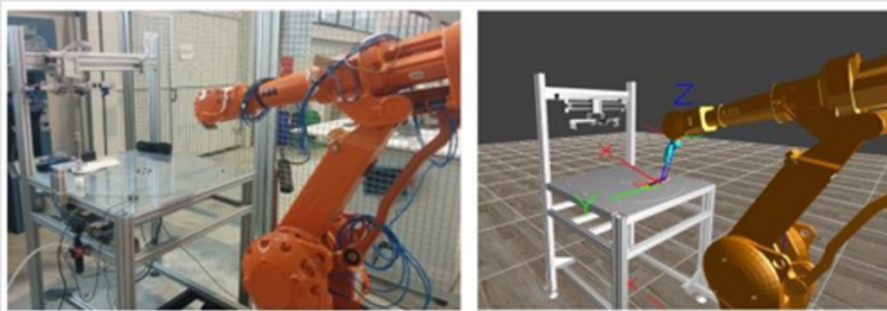
Figure 2: Real and simulated robotic cell.
