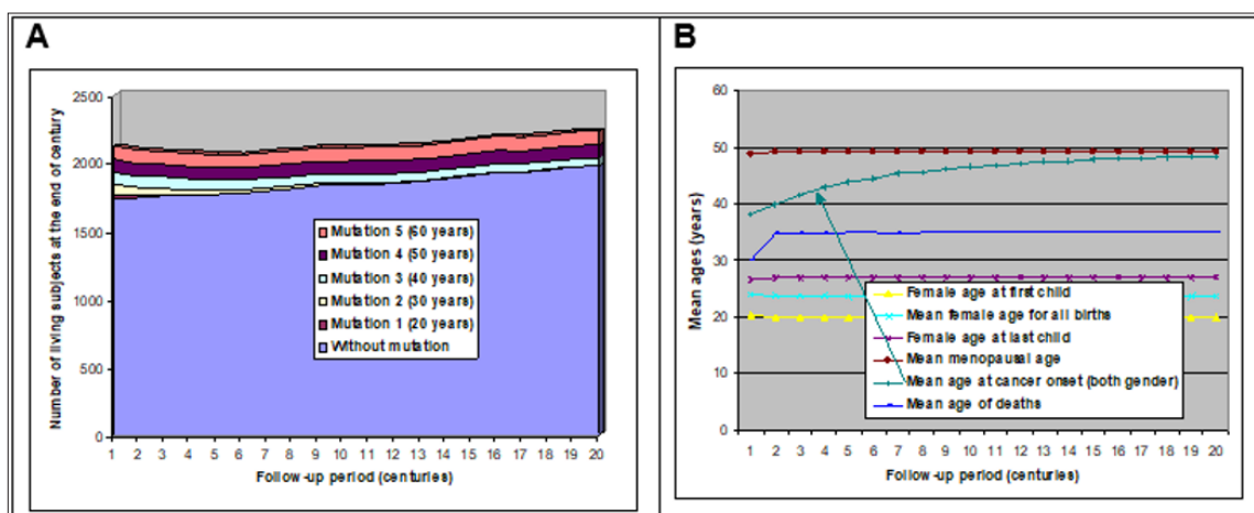
Figure 4: Population evolution according to 5 types of mutation inducing a 50% cancer risk occurring in average at 5 ages [20-60] in men and women (follow-up: 2 millennia).
