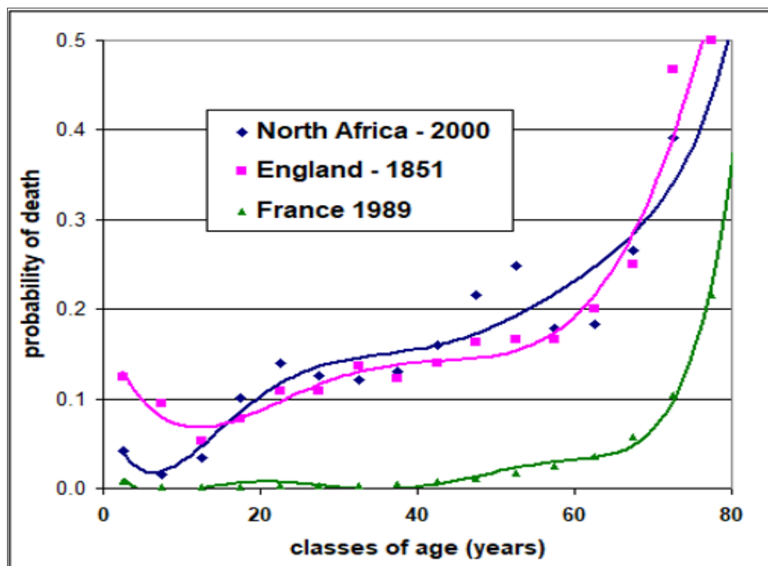
Figure 1: Fitted curves for female mortality by 5-year classes of age and three different contexts.
