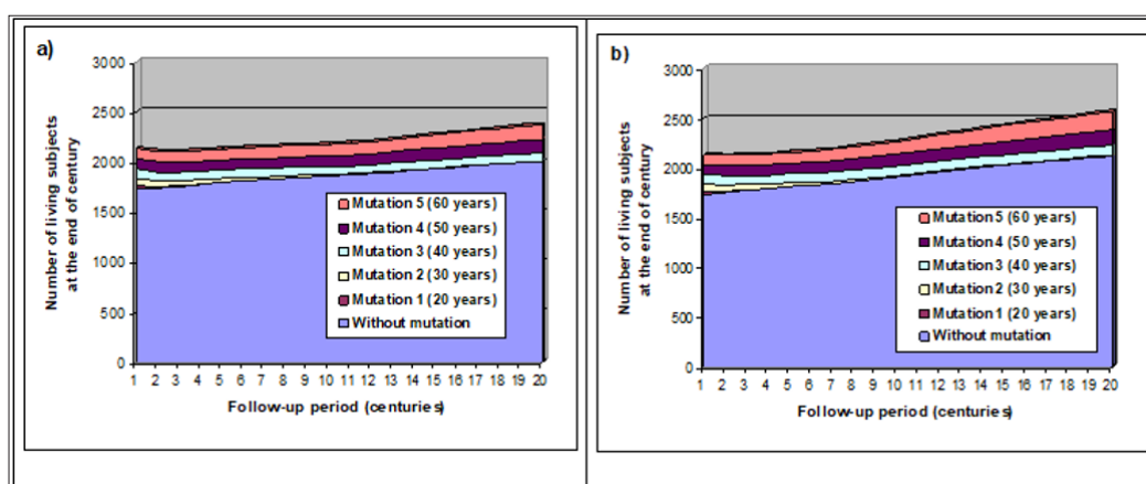
Figure 5: Impact of two types of reproduction advantages.
