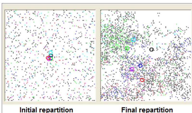
Figure 6: Spontaneous geographic dissemination of 5 mutations increasing cancer risk when individuals carry more than one of them: black points and circle correspond to individual carrying no deleterious mutation. Other circles locate the centroid of mutation carriers.
