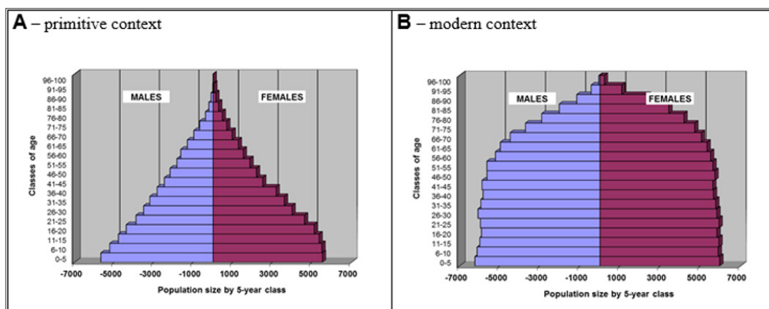
Figure 3: Pyramid of age of the last century after 2 millennia of follow-up resulting from simulations according to two contexts: primitive and modern.
